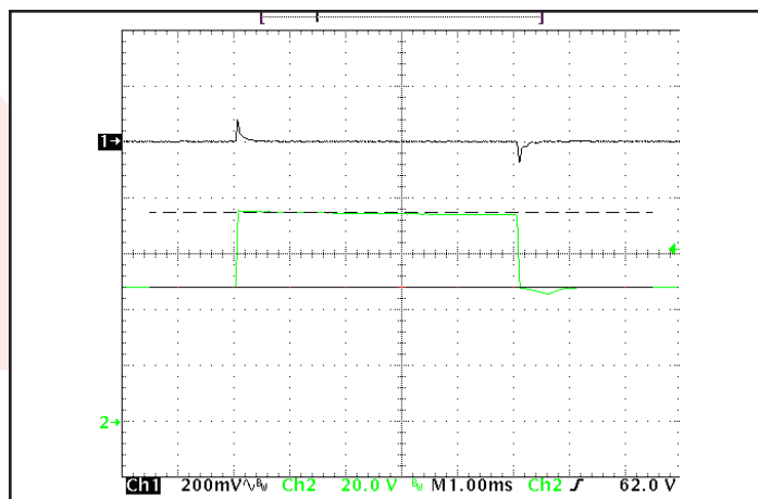
Figure 6: Output voltage response to step-change in input voltage (nominal to maximum input voltage), at full load current. Load cap: 15μF tantalum capacitor and 1μF ceramic cap. Ch 1: Vout, Ch 2: Vin.
