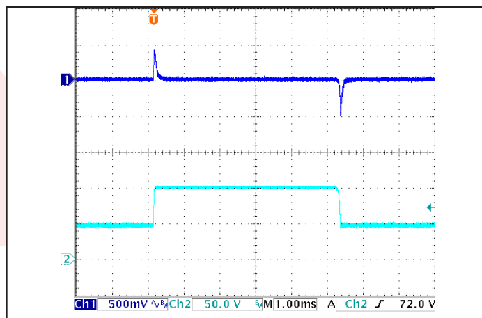
Figure 6: Output voltage response to step-change in input voltage (nominal to maximum input voltage), at full load current. Load cap: uF ceramic cap. Ch 1: Vout, Ch 2: Vin.
