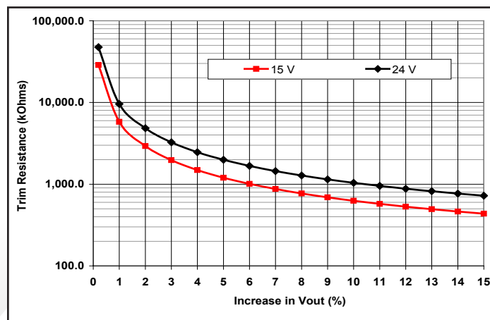
Common Figure 4: Trim graph for trim-up 15 and 24 V outputs.
