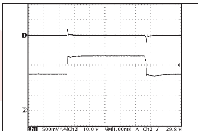
Figure 6: Output voltage response to step-change in input voltage (nominal to maximum), at full load current. Load cap: 15 \mu F tantalum capacitor and 1 \mu F ceramic cap. Ch 1: Vout, Ch 2: Vin.
