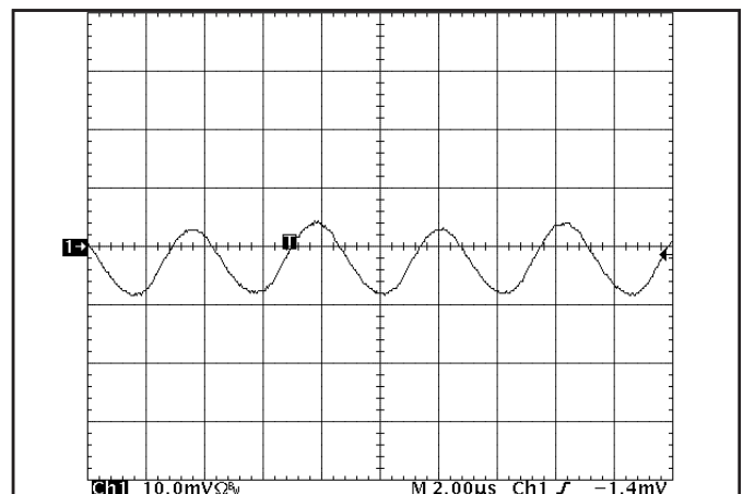
Figure 24: Input Terminal Ripple Current, 1.8V & 3.3V outputs at 50% rated output current and nominal input voltage with 10μH source impedance and 100μF electrolytic capacitor (200 mA/div). (see Fig. 23)
