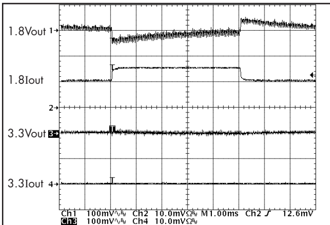
Figure 21: Output voltage response to step-change in Iout1 (50%-75%-50% of I max ; dl/dt = 0.1A/μs). Load cap: 15μF, 300 mΩ ESR tantalum cap & 1μF ceramic cap. Vout (100mV/div), Iout (10A/div). Ch1: Vout1; Ch2 Iout1; Ch 3: Vout2; Ch 4 Iout2
