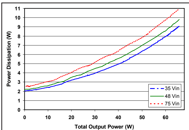
Figure 4: Overall converter power dissipation vs. output power from zero load to full load at minimum, nominal, and maximum input voltage at 25°C. Both loads are equal and range from zero to full load.
