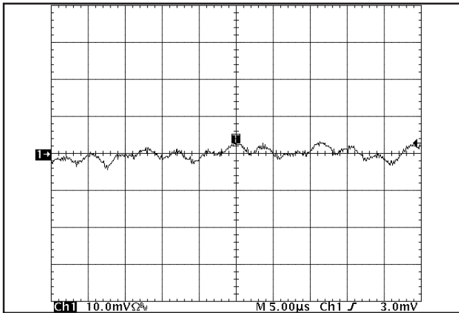
Figure 19: Input Reflected Ripple Current, i_s , through a 10 \mu H source inductor at nominal input voltage and rated load current (5 mA/div). 1.2V and 3.3V outputs at full rated load current. (see Fig. 17)
