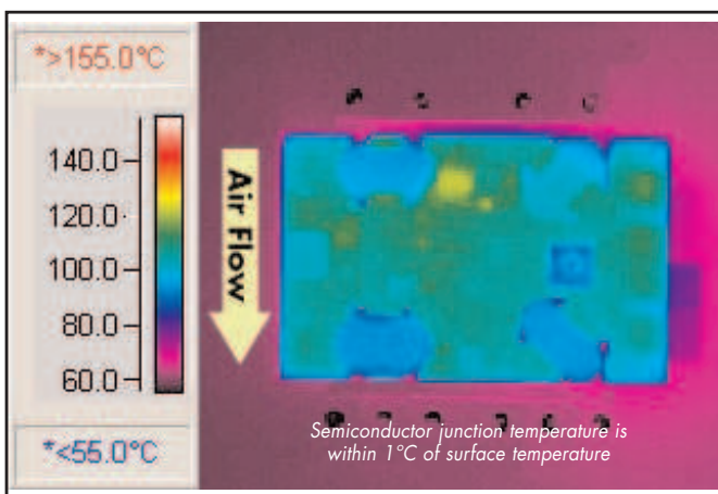
Figure 8: Thermal plot of converter at 15A load on 1.2V output and 15A load on 3.3V output with 55°C air flowing at 200 LFM. Air flow across the converter is from pin 1 to pin 3 (nominal input voltage).
