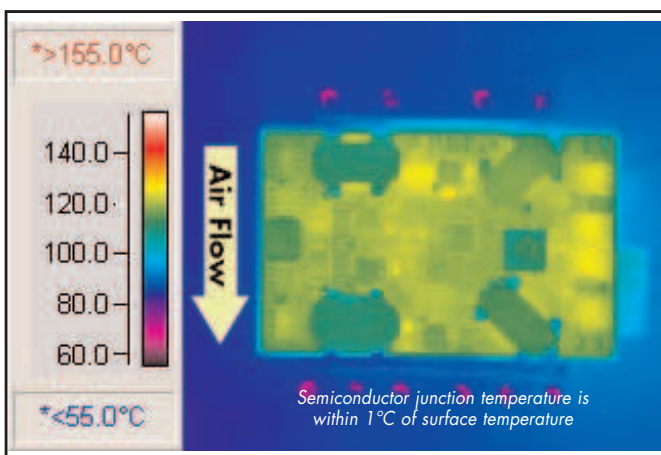
Figure 12: Thermal plot of converter at 15A load on 1.2V output and 10.5A load on 3.3V output with 85°C air flowing at 200 LFM. Air flow across the converter is from pin 1 to pin 3 (nominal input voltage).
