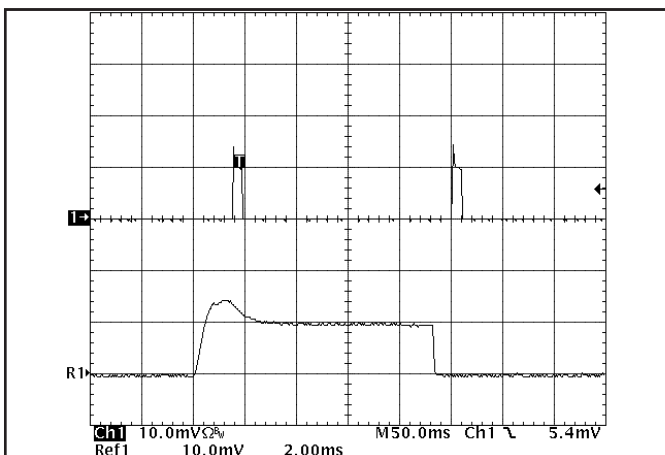
Figure 23: Load current for 1.2V output (20A/div) as a function of time when the converter attempts to turn on into a 10 m \Omega short circuit. Bottom trace is an expansion of the on-time portion of the top trace.
