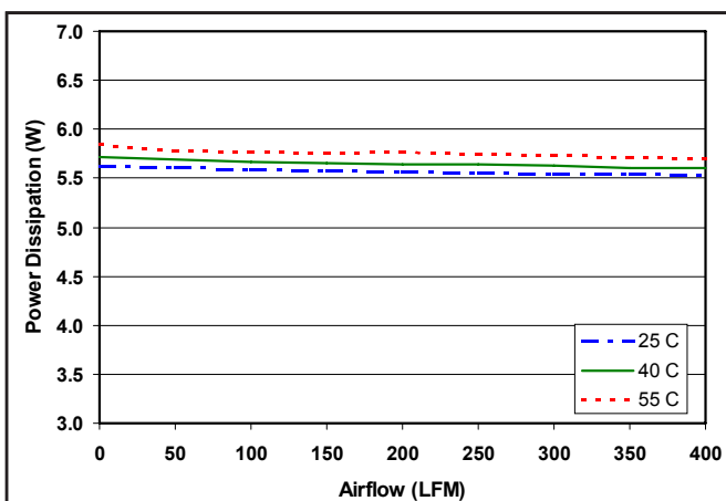
Figure 6: Overall converter power dissipation at nominal output voltages and 60% rated power on each output rail vs. airflow rate for ambient temperatures of 25°C, 40°C and 55°C (nominal input voltage).
