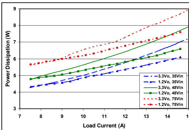
Figure 2: Power dissipation vs. output current, from half load to full load on each output voltage at minimum, nominal, and maximum input voltage at 25°C. Output not under test is held constant at half load.
