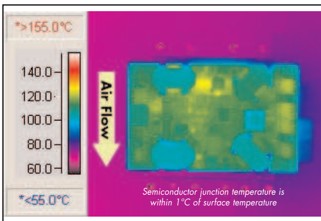
Figure 10: Thermal plot of converter at 15A load on 1.2V output and 13.5A load on 3.3V output with 70°C air flowing at 200 LFM. Air flow across the converter is from pin 1 to pin 3 (nominal input voltage).
