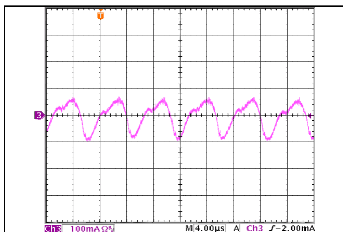
Figure 17: Input Terminal Ripple Current, i_L , at full rated output current and nominal input voltage with 4.7 \mu H source inductor and 100 \mu F electrolytic capacitor (100 mA/div). See Figure 16
