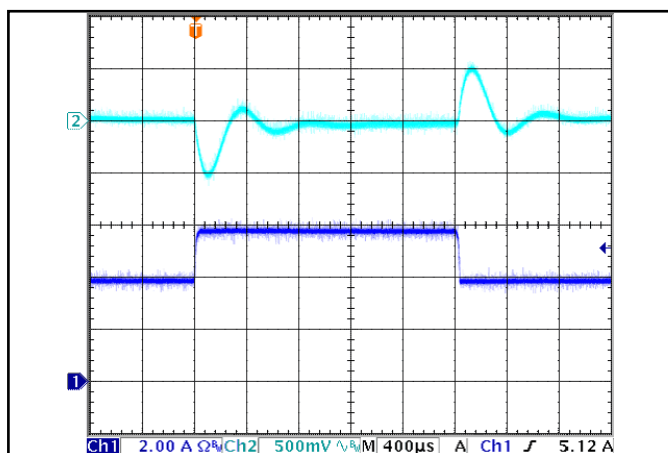
Figure 13: Output voltage response to step-change in load current (50%-75%-50% of I_{out(max)} ; dI/dt = 0.1A/\mu s ). Load cap: 200 \mu F , electrolytic output capacitance. Top trace: Vout (500mV/div), Bottom trace: Iout (2A/div).
