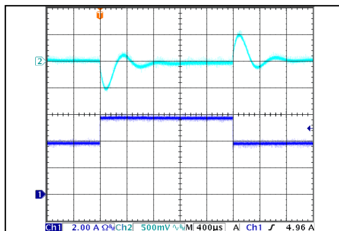
Figure 14: Output voltage response to step-change in load current (50%-75%-50% of I_{out(max)} ; dI/dt = 1A/\mu s ). Load cap: 330 \mu F , electrolytic output capacitance. Top trace: Vout (500mV/div), Bottom trace: Iout (2A/div).
