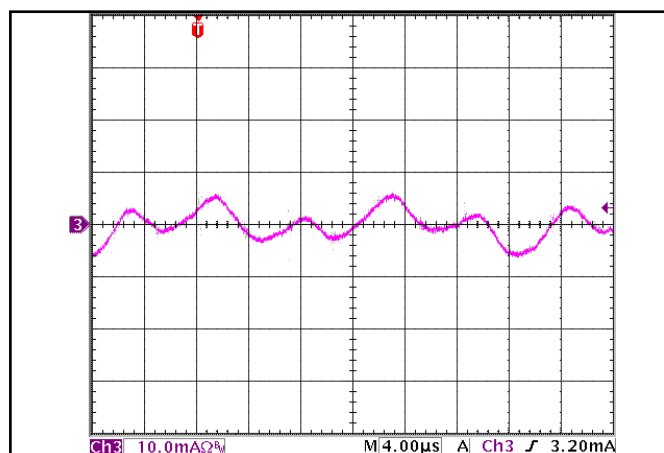
Figure 18: Input reflected ripple current, i_L , through a 4.7 \mu H source inductor at nominal input voltage and rated load current (10 mA/div). (See Figure 16)
