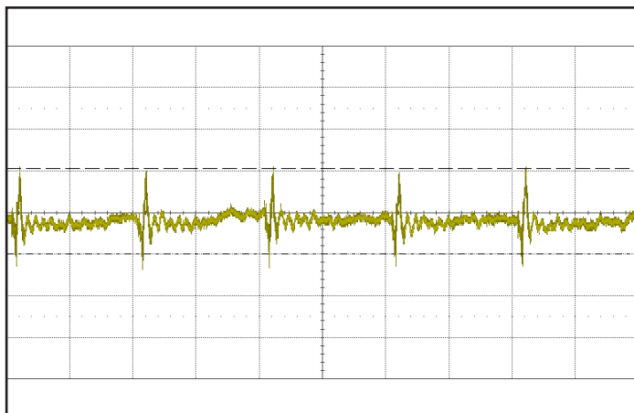
Figure 11: Input reflected ripple current, i_s , through a 4.7 \mu\text{H} source inductor, using a 220 \mu\text{F} input capacitor, at nominal input voltage and rated load current (10 mA/div; 2 \mu\text{s} /div). See Figure 9.
