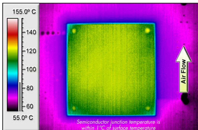
Figure 4: Thermal plot of converter at 36A load current (432W) with 55°C air flowing at the rate of 200LFM. Air is flowing across the converter from pin 4 to pin 1 (nominal input voltage).
