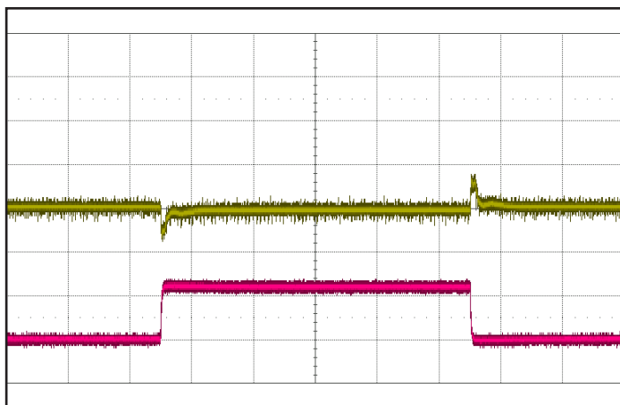
Figure 7: Output voltage response to step-change in load current (50%-75%-50% of I_{out(max)} ; dI/dt = 0.1 \text{ A}/\mu\text{s} ; 1 ms/div). Load cap: 1 \mu\text{F} ceramic and 470 \mu\text{F} electrolytic capacitors. Top trace: V_{out} (500 mV/div). Bottom trace: I_{out} (10 A/div)..
