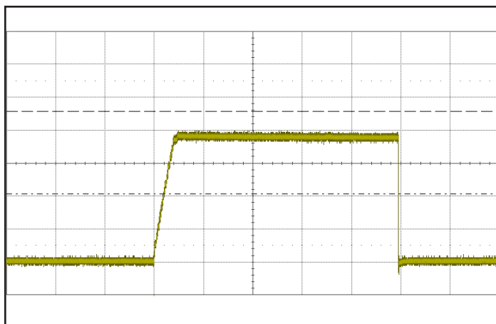
Figure 13: Load current (10 A/div; 10 ms/div) as a function of time when the converter attempts to turn on into a 1 mW short circuit.
