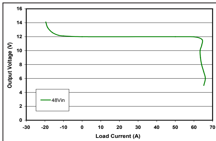
Figure 14: Output voltage vs. load current showing typical current limit curves and OVP shutdown point.
