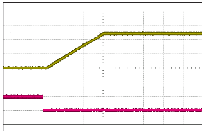
Figure 5: Turn-on transient at full load (resistive load) (10 ms/div). Ch 1: V out (5 V/div) Ch 2: ON/OFF input (5 V/div)
