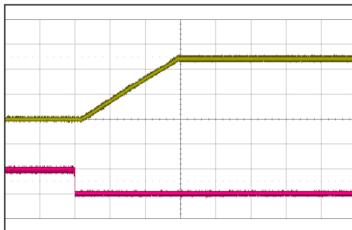
Figure 6: Turn-on transient at zero load (10 ms/div). Ch 1: V out (5 V/div) Ch 2: ON/OFF input (5 V/div)
