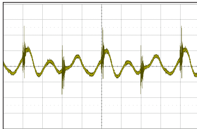
Figure 12: Output voltage ripple at nominal input voltage and rated load current (50 mV/div; 2 \mu\text{s} /div). Load capacitance: 1 \mu\text{F} ceramic capacitor and 15 \mu\text{F} tantalum capacitor. Bandwidth: 20 MHz. See Figure 9.
