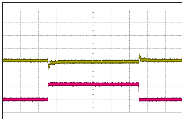
Figure 8: Output voltage response to step-change in load current (50%-75%-50% of I_{out(max)} ; dI/dt = 5 \text{ A}/\mu\text{s} ; 1 ms/div). Load cap: 470 \mu\text{F} electrolytic capacitor. Top trace: V_{out} (500 mV/div). Bottom trace: I_{out} (10 A/div).
