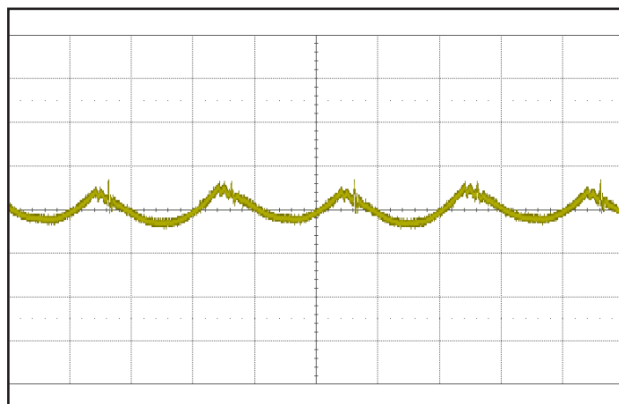
Figure 10: Input Terminal Ripple Current, i_c , at full rated output current and nominal input voltage with 4.7 \mu\text{H} source impedance and 220 \mu\text{F} electrolytic capacitor (1 A/div; 2 \mu\text{s} /div). See Figure 9.
