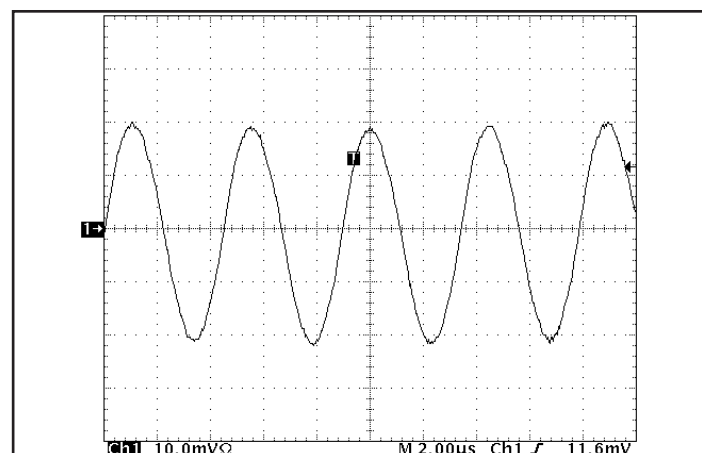
Figure 12: Input Terminal Ripple Current, i_c , at full rated output current and nominal input voltage with 10 \mu H source impedance and 47 \mu F electrolytic capacitor (100mA/div). (See Figure 11).
