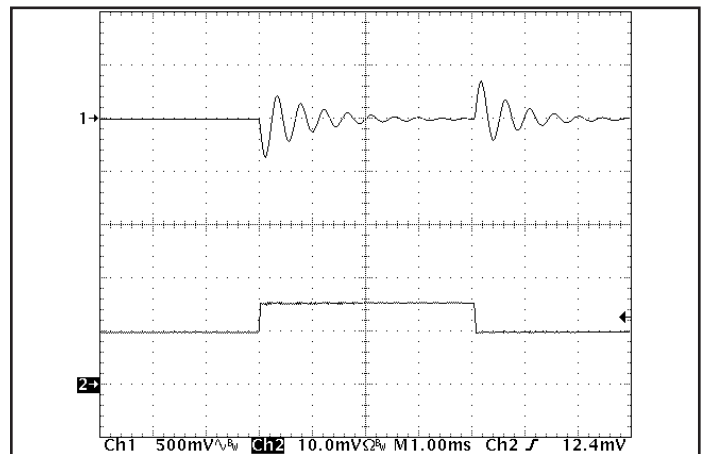
Figure 10: Output voltage response to step-change in load current (50%-75%-50% of I_{out(max)} ; dI/dt = 5A/\mu s ). Load cap: 470 \mu F , 15m \Omega ESR tantalum cap and 1 \mu F ceramic cap. Top trace: Vout (500mV/div), Bottom Trace: Iout (5A/div).
