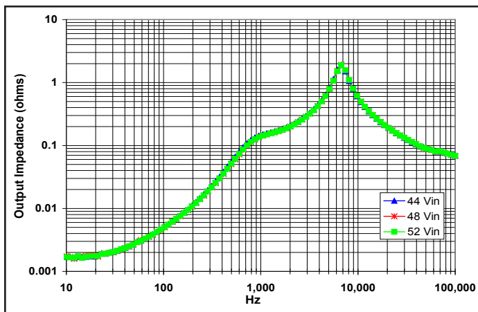
Figure 16: Magnitude of incremental output impedance ( Z_{out} = v_{out}/i_{out} ) for minimum, nominal, and maximum input voltage at full rated power.
