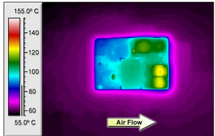
Figure 8: Thermal plot of converter at 24.9 amp load current (37.3W) with 55°C air flowing at the rate of 200 LFM. Air is flowing across the converter from input to output (nominal input voltage).
