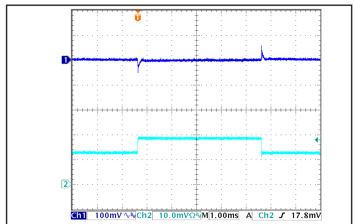
Figure 12: Output voltage response to step-change in load current (50%-75%-50% of I_{out(max)} ; dI/dt = 2A/\mu s ). Load cap: 330 \mu F electrolytic output capacitance. Top trace: V_{out} (100mV/div). Bottom trace: I_{out} (10A/div).
