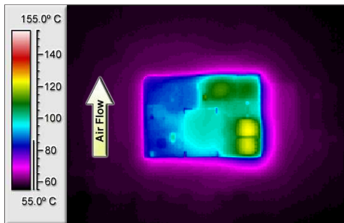
Figure 6: Thermal plot of converter at 25.0 amp load current (37.5W) with 55°C air flowing at the rate of 200 LFM. Air is flowing from pin 3 to pin 1 (nominal input voltage).
