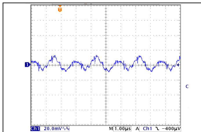
Figure 16: Output voltage ripple at nominal input voltage and rated load current (20 mV/div). Load capacitance: one 1.0\mu F ceramic capacitor and one 100\mu F electrolytic capacitor. Bandwidth: 20 MHz. (See Figure 13).
