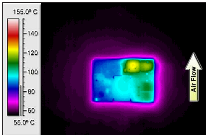
Figure 6: Thermal plot of converter at 15.0 amp load current (49.5W) with 55°C air flowing at the rate of 200 LFM. Air is flowing from pin 3 to pin 1 (nominal input voltage).
