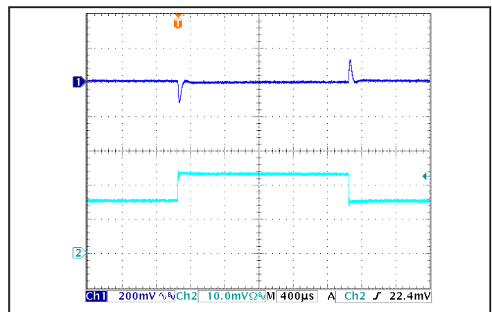
Figure 12: Output voltage response to step-change in load current (50%-75%-50% of I_{out(max)} ; dI/dt = 2A/\mu s ). Load cap: 330 μF electrolytic output capacitance. Top trace: V_{out} (200mV/div). Bottom trace: I_{out} (5A/div).
