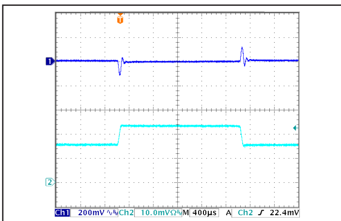
Figure 11: Output voltage response to step-change in load current (50%-75%-50% of I_{out(max)} ; dI/dt = 0.1A/\mu s ). Load cap: 100 μF electrolytic output capacitance. Top trace: V_{out} (200mV/div). Bottom trace: I_{out} (5A/div).
