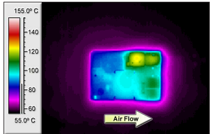
Figure 8: Thermal plot of converter at 15.0 amp load current (49.5W) with 55°C air flowing at the rate of 200 LFM. Air is flowing across the converter from input to output (nominal input voltage).
