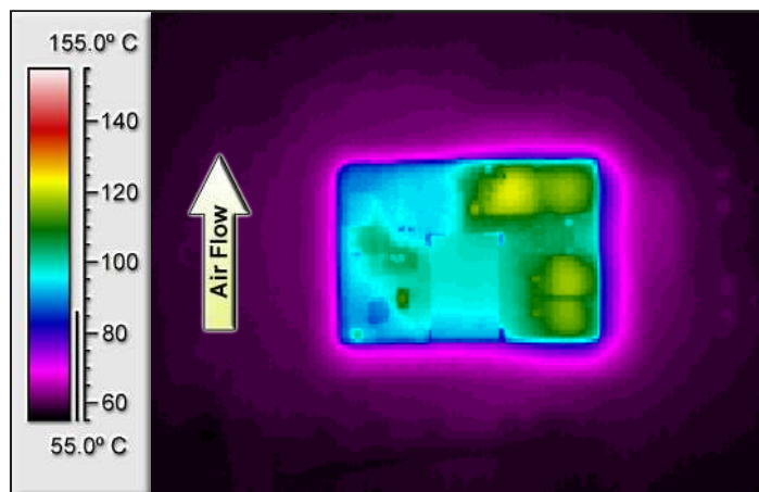
Figure 6: Thermal plot of converter at 20.0 amp load current (50.0W) with 55°C air flowing at the rate of 200 LFM. Air is flowing from pin 3 to pin 1 (nominal input voltage).
