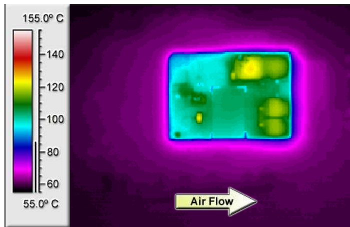
Figure 8: Thermal plot of converter at 20.0 amp load current (50.0W) with 55°C air flowing at the rate of 200 LFM. Air is flowing across the converter from input to output (nominal input voltage).
