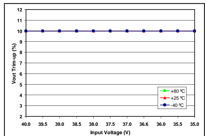
Figure 18: Maximum trim up vs. input voltage at different temperatures V_{in} =35.0~40.0 V.
