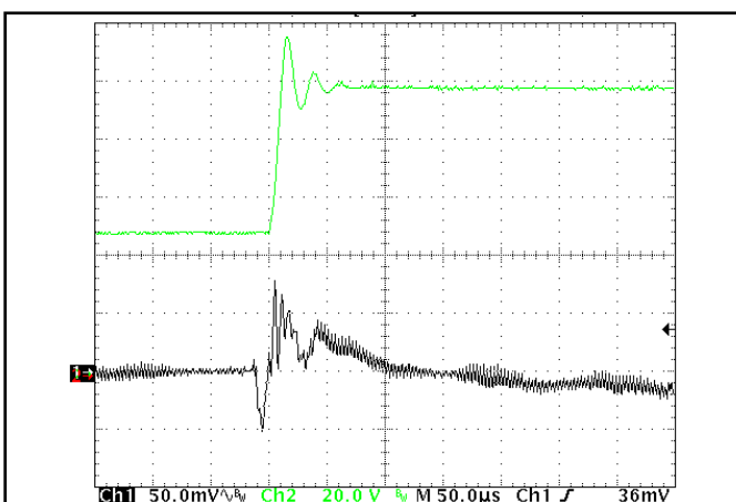
Figure 17: Output voltage response to step-change in input voltage (50V to 100V in 8 \mu S), at 17.5A load current. Load cap: 15 \mu F 100m \Omega ESR tantalum capacitor and 1 \mu F ceramic cap. Ch 1: V_{out} (50mV/div), Ch 2: V_{in} (20V/div).
