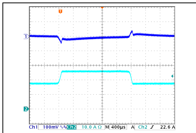
Figure 12: Output voltage response to step-change in load current (50%-75%-50% of I_{out(max)} ; dI/dt = 0.3 A/\mu s ). Load cap: 10uF, 100 mΩ ESR tantalum cap and 1uF ceramic cap. Ch 1: V_{out} (100mV/div), Ch 2: I_{out} (10A/div).
