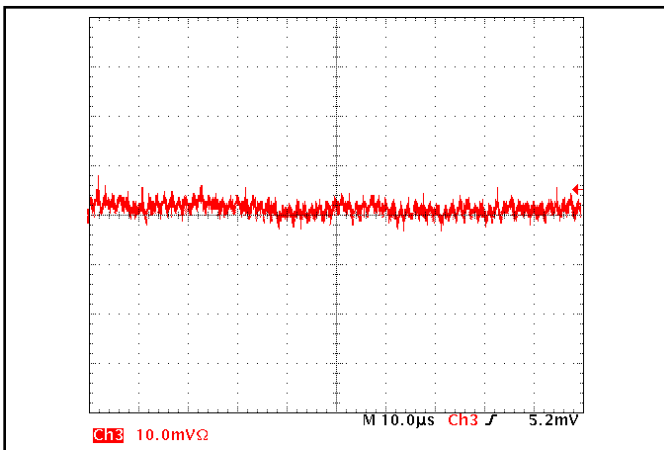
Figure 15: Input reflected ripple current, i_s , through a 10 \mu H source inductor, using a 47 \mu F electrolytic input capacitor (2mA/div). Bandwidth: 250MHz. See Figure 13.
