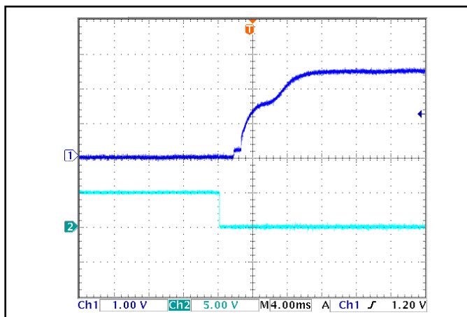
Figure 9: Turn-on transient at full load (resistive load) (4 ms/div). Load cap: 10uF, 100 mΩ ESR tantalum capacitor and 1uF ceramic capacitor. Input voltage pre-applied. Ch 1: V_{out} (1V/div), Ch 2: ON/OFF input (5V/div).
