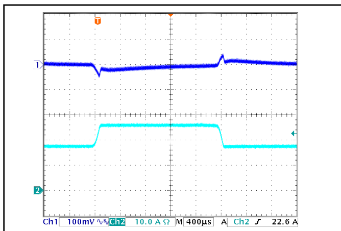
Figure 11: Output voltage response to step-change in load current (50%-75%-50% of I_{out(max)} ; dI/dt = 0.1 A/\mu s ). Load cap: 10uF, 100 mΩ ESR tantalum cap and 1uF ceramic cap. Ch 1: V_{out} (100mV/div), Ch 2: I_{out} (10A/div).
