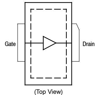
Figure 1. Pin Connections
