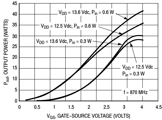
Figure 7. CW Output Power versus Gate-Source Voltage
