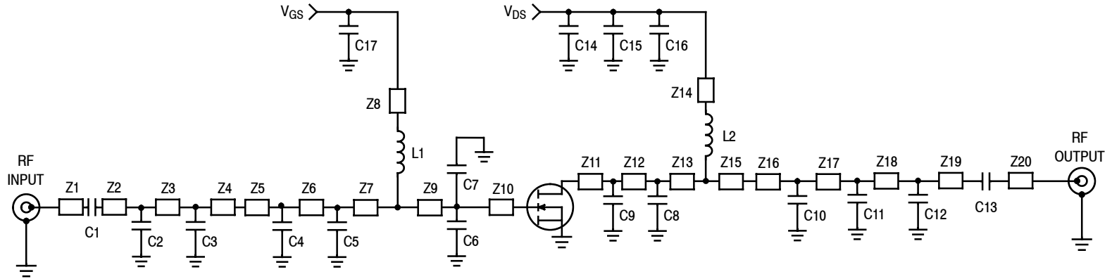
Figure 11. AFT09MS031NR1 Broadband Reference Circuit Schematic — 760–870 MHz
