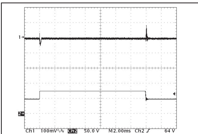
Figure 17: Output voltage response to step-change in input voltage (48V to 75V), at 20A load current. Load cap: 15\ \mu\text{F} tantalum capacitor and 1\ \mu\text{F} ceramic cap. Ch 1: V_{\text{out}} (100mV/div), Ch 2: V_{\text{in}} (50V/div).
