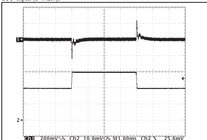
Figure 11: Output voltage response to step-change in load current (50%-75%-50% of I_{out(max)} ; dI/dt = 0.1A/\mu s ). Load cap: 15 \mu F tantalum cap and 1 \mu F ceramic cap. Ch 1: V_{out} (200mV/div), Ch 2: I_{out} (5A/div).
