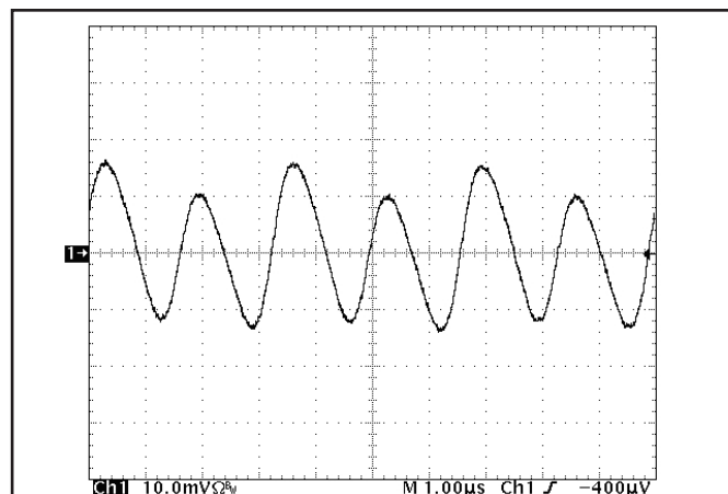
Figure 14: Input Terminal Ripple Current, i_c , at full rated output current and nominal input voltage with 10\mu H source impedance and 47\mu F electrolytic capacitor (50 mA/div). See Figure 13.
