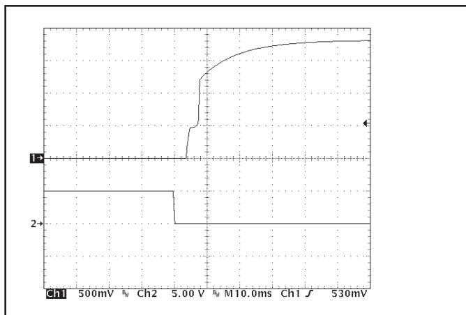
Figure 9: Turn-on transient at full load (resistive load) (10 ms/div). Load cap: 10 \mu F, 100 m \Omega ESR tantalum capacitor and 1 \mu F ceramic capacitor. Input voltage pre-applied. Ch 1: V_{out} (500 mV/div), Ch 2: ON/OFF input (5 V/div).
