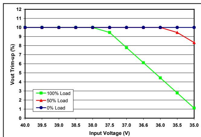
Figure 18: Achievable trim-up percentage vs. input voltage at 0%, 50% and full load. V_{in}=35-40V .
