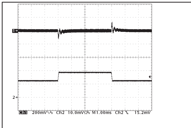
Figure 11: Output voltage response to step-change in load current (50%-75%-50% of I_{out(max)} ; dI/dt = 0.1A/\mu s ). Load cap: 15 \mu F tantalum cap and 1 \mu F ceramic cap. Ch 1: V_{out} (200 mV/div), Ch 2: I_{out} (10 A/div).
