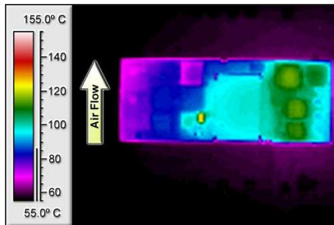
Figure 8: Thermal plot of converter at 22.6A load current (40.68 W) with 55°C air flowing at the rate of 200 LFM. Air is flowing across the converter from input to output (nominal input voltage).
