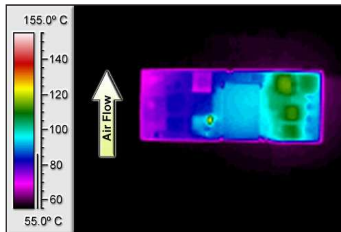
Figure 6: Thermal plot of converter at 24 A load current (43.2W) with 55°C air flowing at the rate of 200 LFM. Air is flowing across the converter from pin 3 to pin 1 (nominal input voltage).
