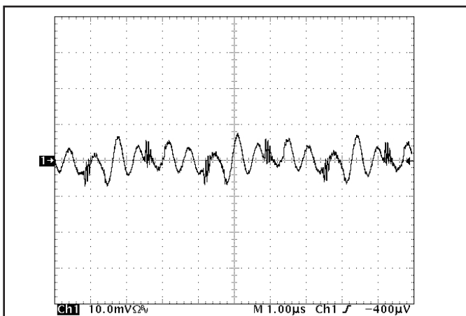
Figure 15: Input reflected ripple current, i_s , through a 10\mu H source inductor, using a 47\mu F electrolytic input capacitor (5mA/div). See Figure 13.
