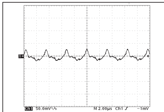
Figure 16: Output voltage ripple at nominal input voltage and rated load current (50 mV/div). Load capacitance: 1\mu F ceramic capacitor and 15\mu F tantalum capacitor. Bandwidth: 20 MHz. See Figure 13.
