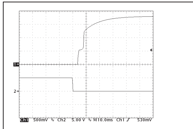
Figure 10: Turn-on transient at zero load (10 ms/div). Load cap: 10 \mu F, 100 m \Omega ESR tantalum capacitor and 1 \mu F ceramic capacitor. Ch 1: V_{out} (500 mV/div), Ch 2: ON/OFF input (5 V/div).
