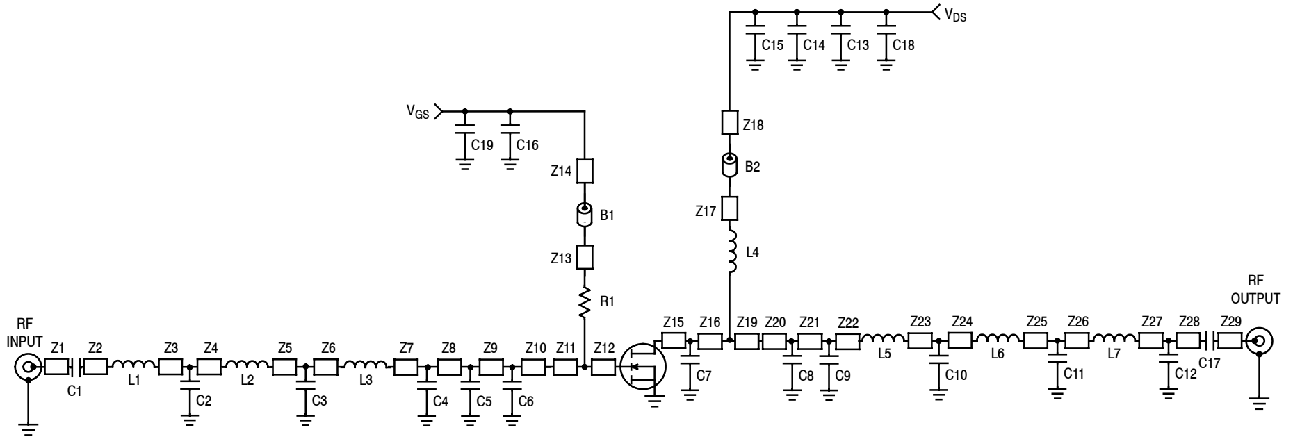
Figure 18. AFT05MS031NR1 UHF Wideband Reference Circuit Schematic — 450-520 MHz
