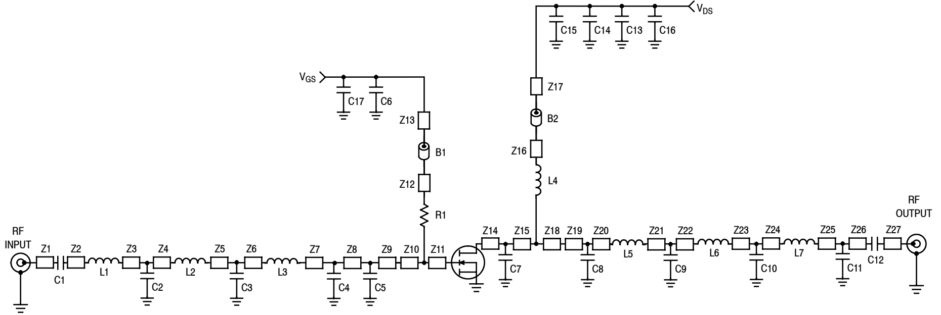
Figure 11. AFT05MS031NR1 UHF Wideband Reference Circuit Schematic — 380-450 MHz
