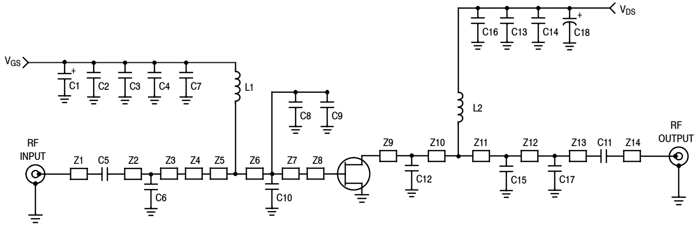
Figure 6. AFT05MS031NR1 Narrowband Test Circuit Schematic — 520 MHz
