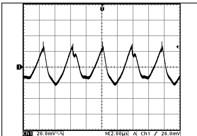
Figure 16: Output voltage ripple at nominal input voltage and rated load current (20 mV/div). Load capacitance: 1 \mu F ceramic capacitor and 15 \mu F tantalum capacitor. Bandwidth: 20 MHz. See Figure 13.
