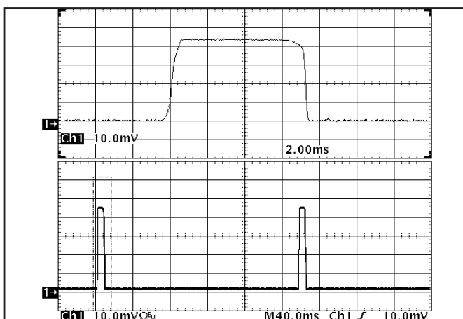
Figure 18: Load current (5A/div) as a function of time when the converter attempts to turn on into a 1 m \Omega short circuit. Top trace (2ms/div) is an expansion of the on-time portion of the bottom trace.
