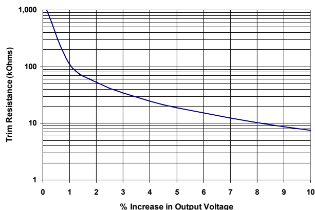
Figure C: Trim Up Graph for 1.5V out
