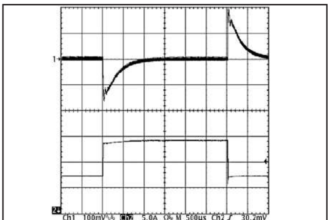
Figure 12: Output voltage response to step-change in load current (50%-75%-50% of I_{max} ; dI/dt = 5A/\mu s ). Load cap: 470 μF, 30 mΩ ESR tantalum capacitor and 1 μF ceramic capacitor. Top trace: V_{out} (100mV/div), Bottom trace: I_{out} (5A/div).
