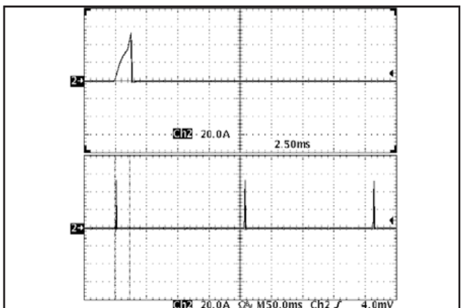
Figure 18: Load current (20A/div) as a function of time when the converter attempts to turn on into a 10\ m\Omega short circuit. Top trace is an expansion of the on-time portion of the bottom trace.
