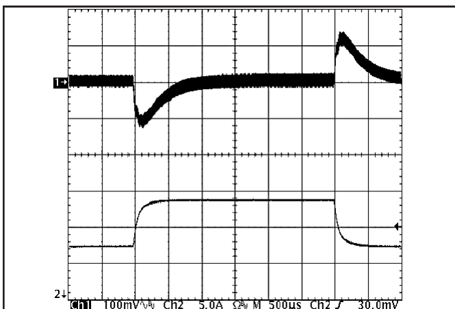
Figure 11: Output voltage response to step-change in load current (50%-75%-50% of I_{max} ; dI/dt = 0.1A/\mu s ). Load cap: 10 μF, 100 mΩ ESR tantalum capacitor and 1 μF ceramic capacitor. Top trace: V_{out} (100mV/div), Bottom trace: I_{out} (5A/div).
