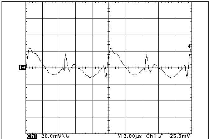
Figure 16: Output voltage ripple at nominal input voltage and rated load current (20 mV/div). Load capacitance: 1\ \mu F ceramic capacitor and 10\ \mu F tantalum capacitor. Bandwidth: 20 MHz. (See Figure 13).
