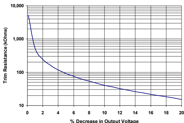
Figure B: Trim Down Graph for 1.5V out
