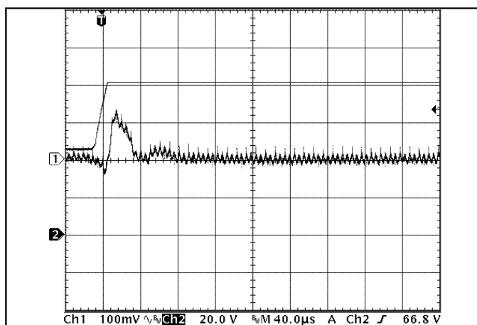
Figure 17: Output voltage response to step-change in input voltage (50V to 100V in 20 μs). Load cap: 10\ \mu\text{F} , 100\text{m}\Omega ESR tantalum capacitor and 1\ \mu\text{F} ceramic cap. Ch 1: V_{out} (100mV/div), Ch 2: V_{in} (20V/div).
