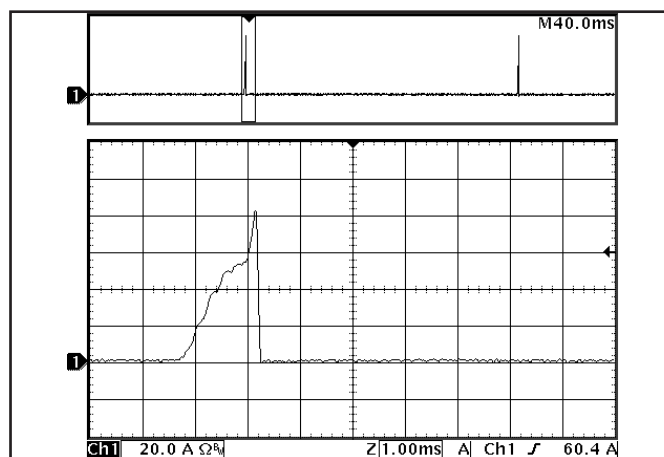
Figure 18: Load current (20A/div) as a function of time when the converter attempts to turn on into a 1\text{m}\Omega short circuit. Bottom trace (1ms/div) is an expansion of the on-time portion of the top trace.
