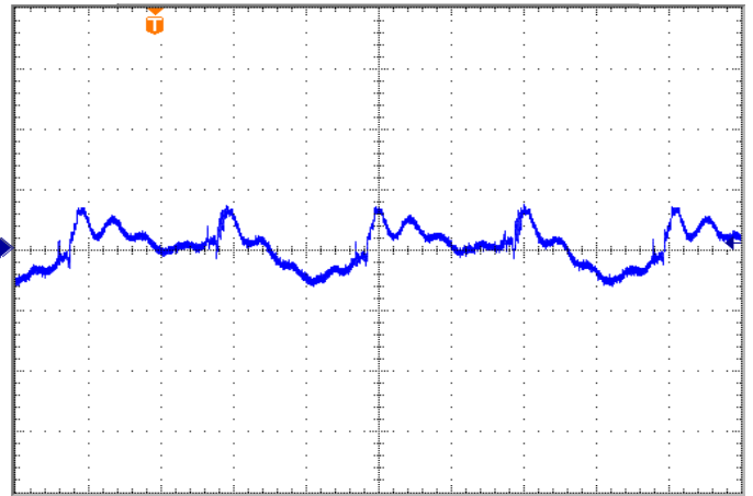
Figure 16: Output Ripple voltage at nominal input voltage and rated load current (200 mV/div, 2\mu s /div). Load capacitance: 1\mu F ceramic and 15\mu F tantalum output capacitors. Bandwidth: 20 MHz. (See Figure 13).
