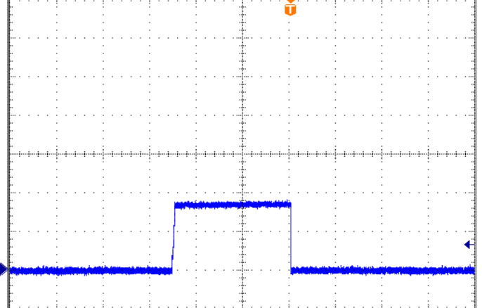
Figure 18: Output Short Load Current (20A/div) as a function of time when the converter attempts to turn on into a 1 m\Omega short circuit (20ms/div).
