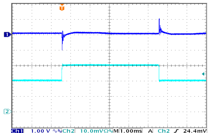
Figure 12: Output Voltage Response to Step-Change in Load Current (50%-75%-50% of Iout(max); dI/dt = 2A/μs). Load cap: 15μF tantalum output capacitance. Top trace: Vout (1V/div). Bottom trace: Iout (10A/div).
