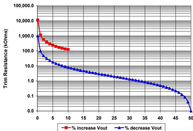
Figure C: Trim Graph
