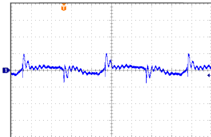
Figure 16: Output Ripple voltage at nominal input voltage and rated load current (100 mV/div, 2µs/div). Load capacitance: one 1.0µF ceramic capacitor and one 15µF tantalum capacitor. Bandwidth: 20 MHz. (See Figure 13).
