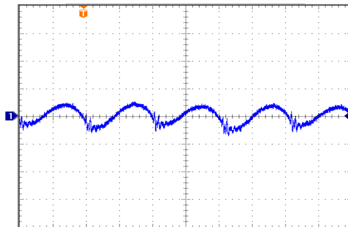
Figure 14: Input Terminal Ripple Current, i_c , at full rated output current and nominal input voltage with 4.7 µH source impedance and 220 µF electrolytic capacitor (Ch.1 200mA/div, 2 µs/div). (See Figure 13).
