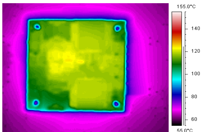
Figure 6: Thermal Image of converter at 33 amp load current (396W) with 55°C air flowing at the rate of 200 LFM. Air is flowing from pin 4 to pin 1 (nominal input voltage).
