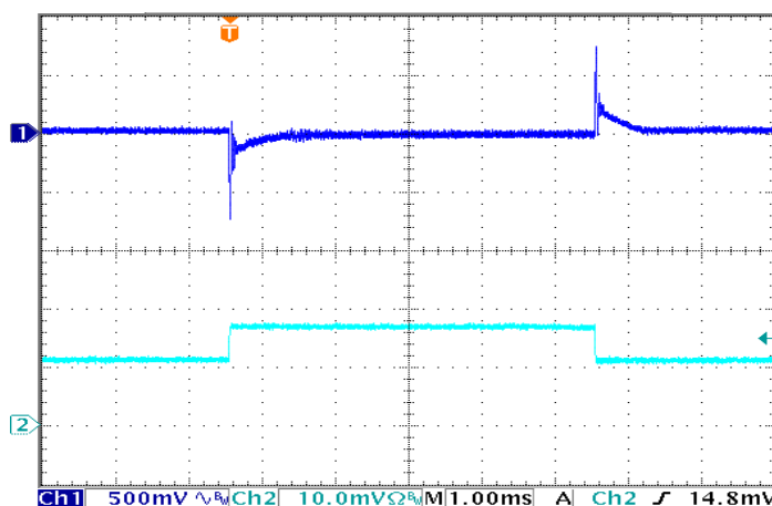
Figure 12: Output Voltage Response to Step-Change in Load Current (50%-75%-50% of Iout(max); dI/dt = 2A/μs). Load cap: 15μF tantalum output capacitance. Top trace: Vout (500mV/div). Bottom trace: Iout (20A/div).
