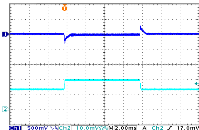
Figure 11: Output Voltage Response to Step-Change in Load Current (50%-75%-50% of Iout(max); dI/dt = 0.1A/μs). Load cap: 15μF tantalum output capacitance. Top trace: Vout (500mV/div). Bottom trace: Iout (20A/div).
