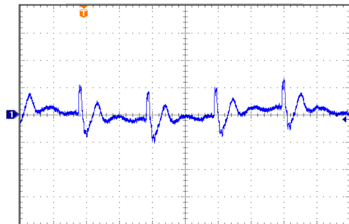
Figure 15: Input Reflected Ripple Current, i_s , through a 4.7 µH source inductor at nominal input voltage and rated load current (20 mA/div, 2 µs/div). (See Figure 13).
