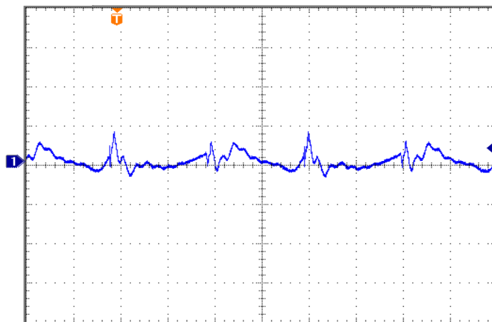
Figure 16: Output Ripple voltage at nominal input voltage and rated load current (200 mV/div, 2 µs/div). Load capacitance: one 1.0 µF ceramic capacitor and one 15 µF tantalum capacitor. Bandwidth: 20 MHz. (See Figure 13).
