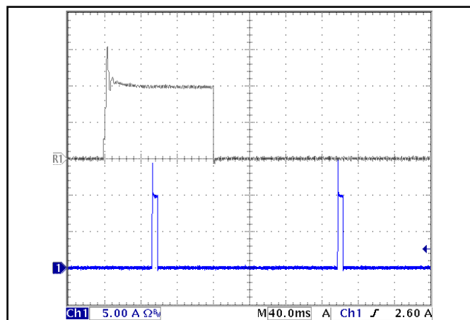
Figure 22: Load current (5A/div) as a function of time when the converter attempts to turn on into a 10 m\Omega short circuit. Top trace (40ms/div) is an expansion of the on-time portion of the bottom trace.
