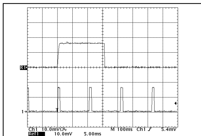
Figure 22: Load current (20A/div) as a function of time when the converter attempts to turn on into a 10 m\Omega short circuit. Top trace (5ms/div) is an expansion of the on-time portion of the bottom trace.
