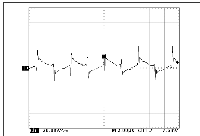
Figure 20: Output voltage ripple at nominal input voltage and rated load current (20 mV/div). Load capacitance: 1 \mu F ceramic capacitor and 10 \mu F tantalum capacitor. Bandwidth: 20 MHz. See Figure 17.
