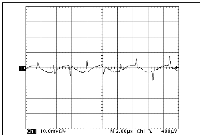
Figure 19: Input reflected ripple current, i_s , through a 10 \mu H source inductor at nominal input voltage and rated load current (20 mA/div). See Figure 17.
