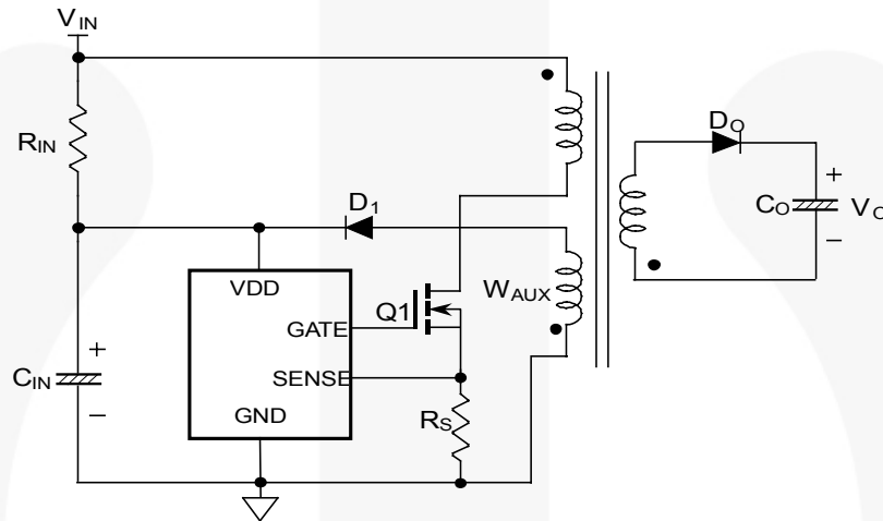
Figure 1. Typical Application
