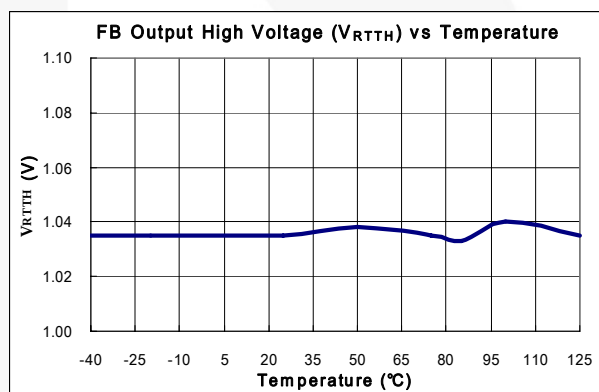
Figure 15. FB Output High Voltage (V RTTH ) vs. Temperature
