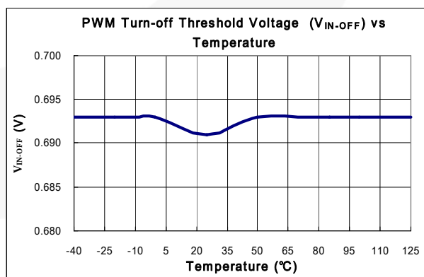
Figure 17. PWM Turn-off Threshold Voltage (V IN-OFF ) vs. Temperature
