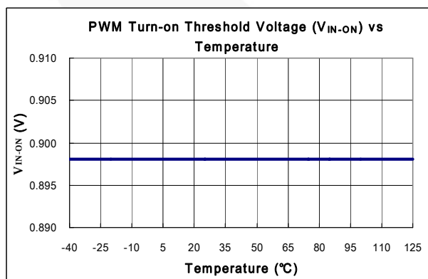
Figure 16. PWM Turn-on Threshold Voltage (V IN-ON ) vs. Temperature
