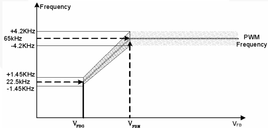
Figure 5. PWM Frequency
