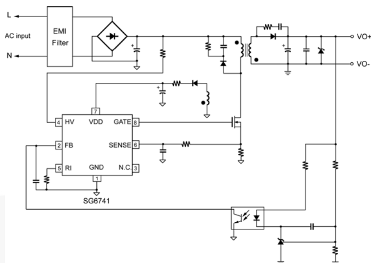
Figure 1. Typical Application
