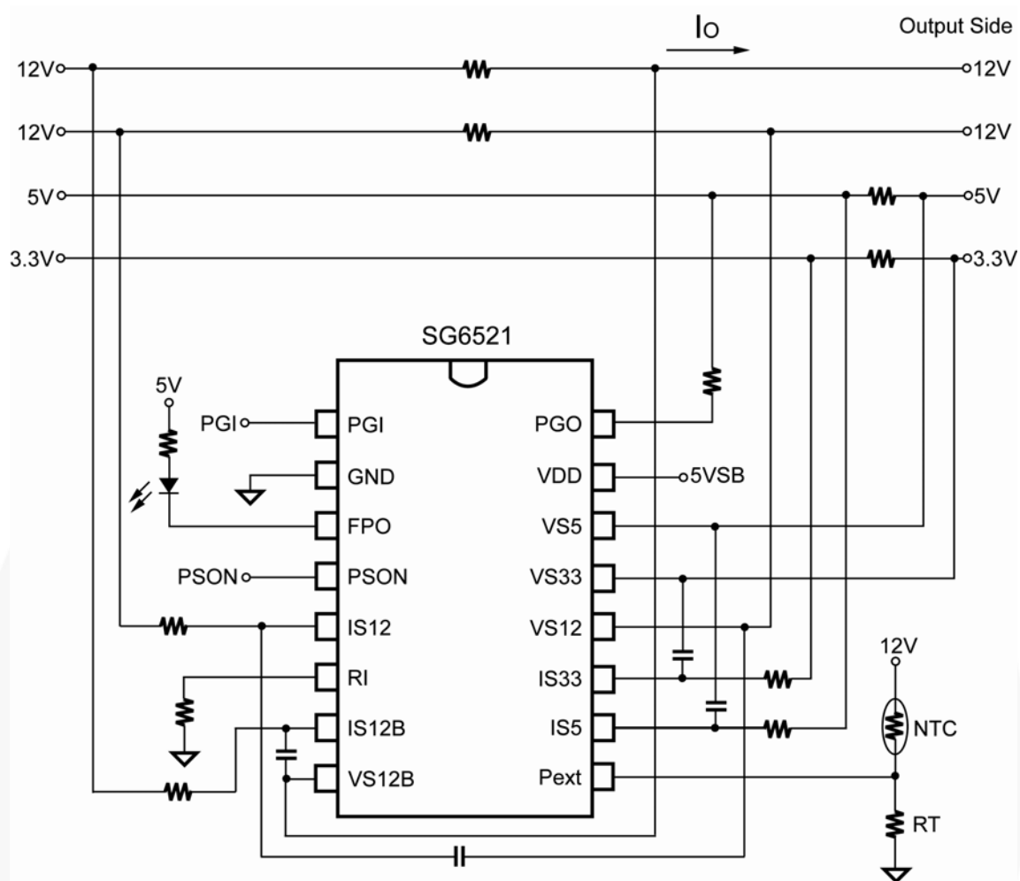
Figure 1. Typical Application
