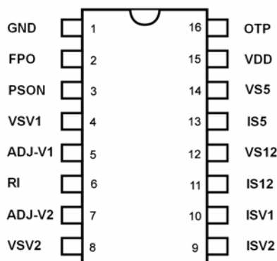
Figure 3. Pin Configuration
