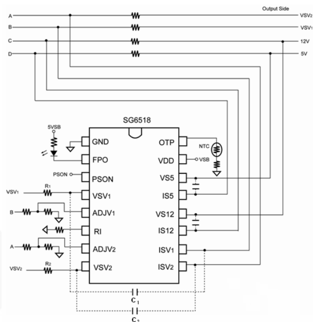
Figure 1. Typical Application
