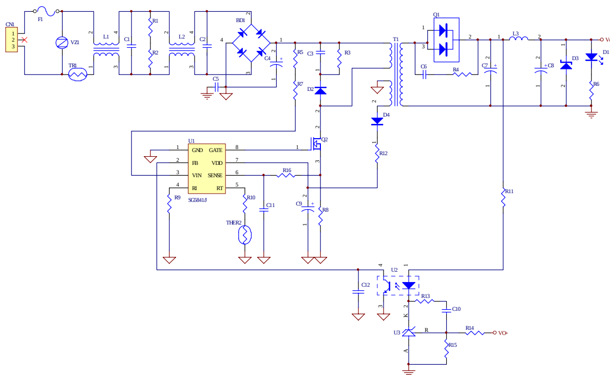
Figure 15. Reference Circuit
