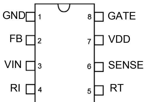
Figure 4. Pin Configuration
