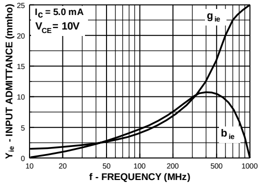
Input Admittance vs Frequency-Output Short Circuit
