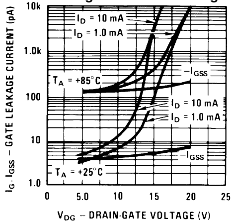
Leakage Current vs. Voltage
