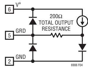
Figure 4. GRD Pin
