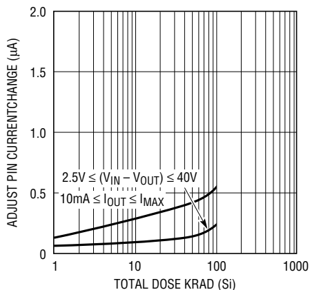
Adjust Pin Current Change
