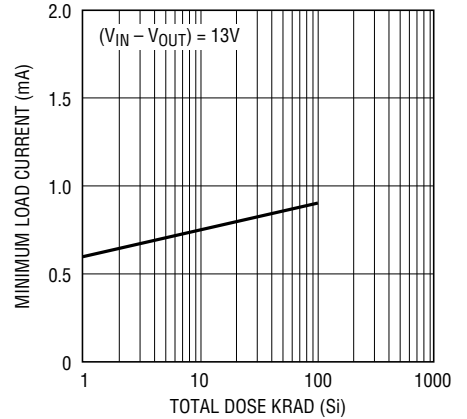
Minimum Load Current
