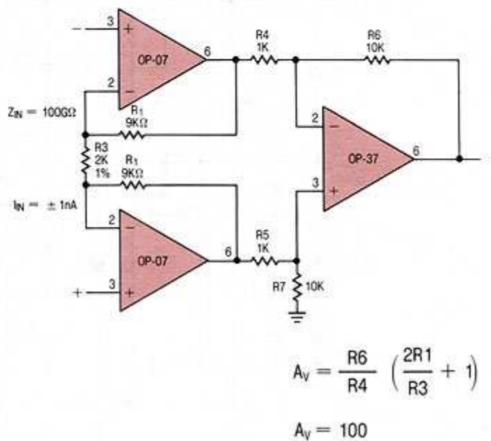
Instrumentation Amplifier
