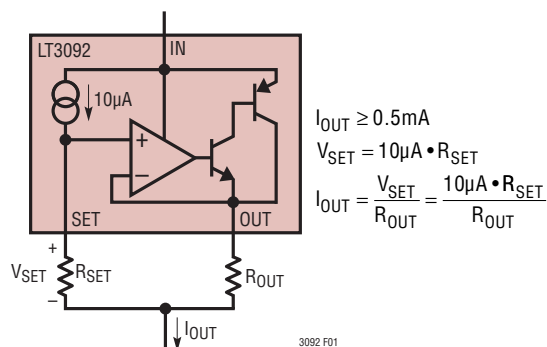
Figure 1. Using the LT3092 as a Current Source
