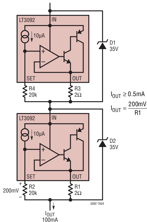
High Voltage Current Source
