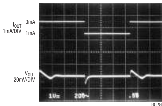
Figure 1. 1mA Load Step with C L = 1μF
