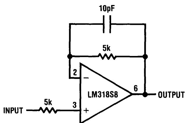
Voltage Follower
