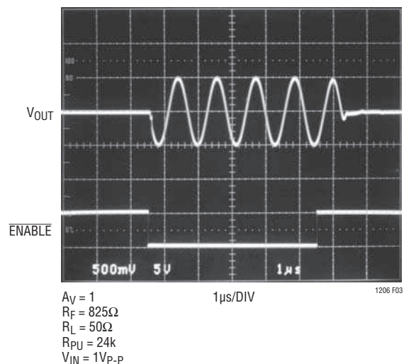
Figure 3. Shutdown Operation
