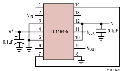
8th Order Butterworth Lowpass Filter f_{\text{CLK}}/f_c = 100:1
