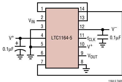
8th Order Butterworth Lowpass Filter f_{\text{CLK}}/f_c = 50:1
