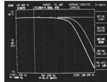
Amplitude Response
