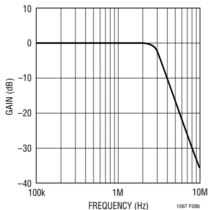
Gain Response
