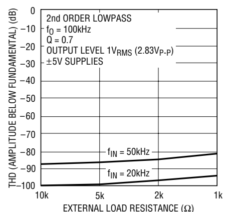
Distortion vs External Load Resistance ( V_S = \pm 5V , 25°C) (Figure 8)
