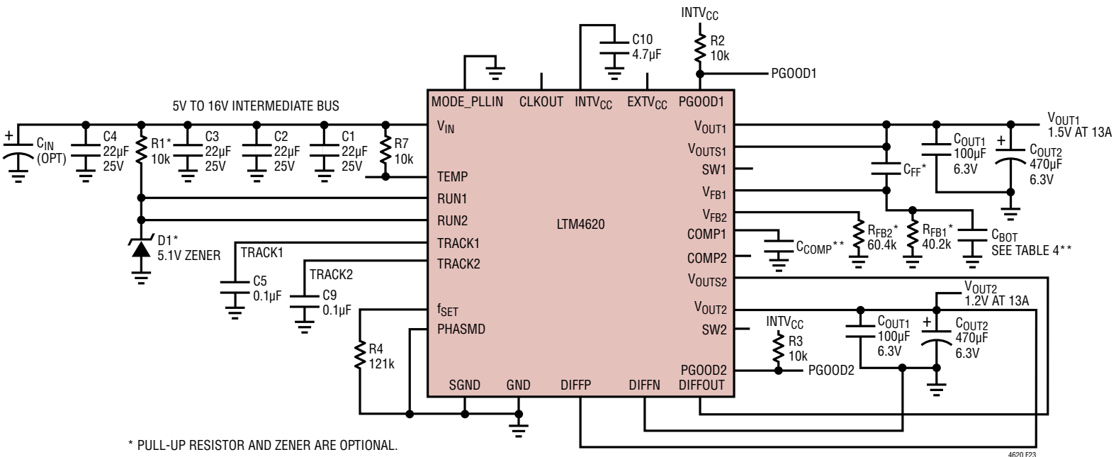
Figure 23. Typical 5V IN to 16V IN , 1.5V and 1.2V Outputs
