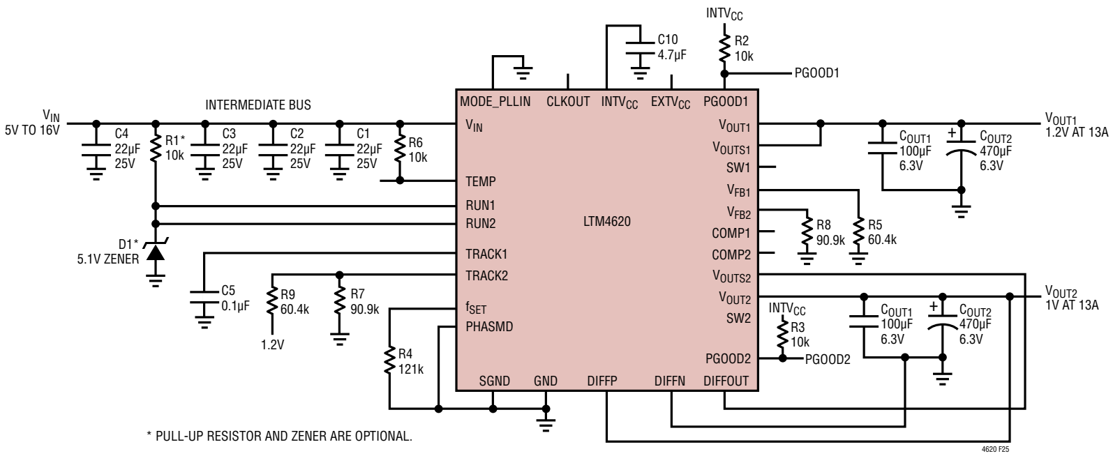
Figure 25. LTM4620 1.2V and 1V Output Tracking
