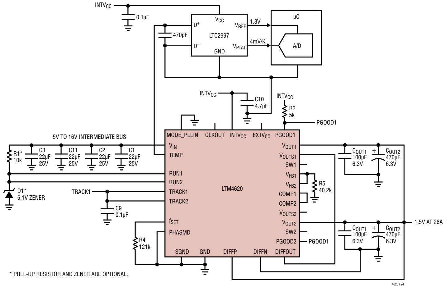
Figure 24. LTM4620 2-Phase, 1.5V at 26A Design with Temperature Monitoring
