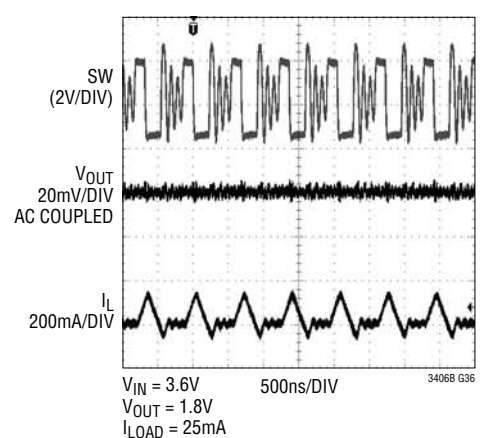
Discontinuous Operation
