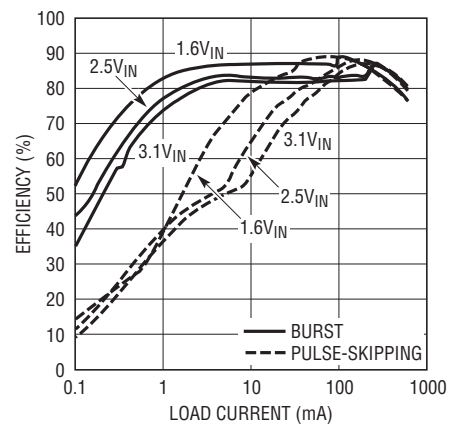
Efficiency vs Load Current, V_{OUT} = 1.2\text{V}
