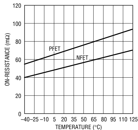
Switch On-Resistance vs Temperature, V_{IN} = 3.3\text{V}
