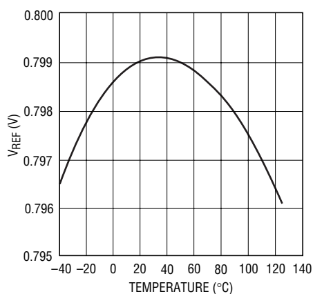
V_{REF} vs Temperature, V_{IN} = 3.3\text{V}
