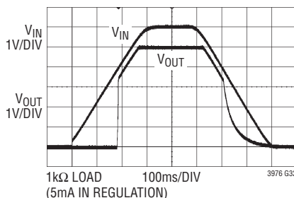
Start-Up/Dropout Performance
