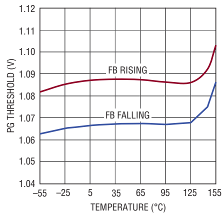
PG Thresholds
