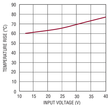
Figure 11. Temperature Rise of the LT3976 at 5A in the Front Page Application
