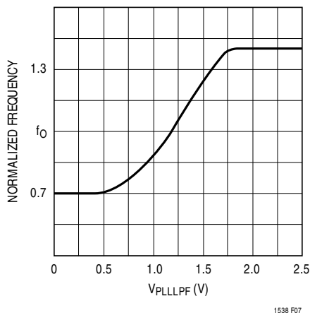
Figure 7. Operating Frequency vs V_{\text{PLLLPF}}
