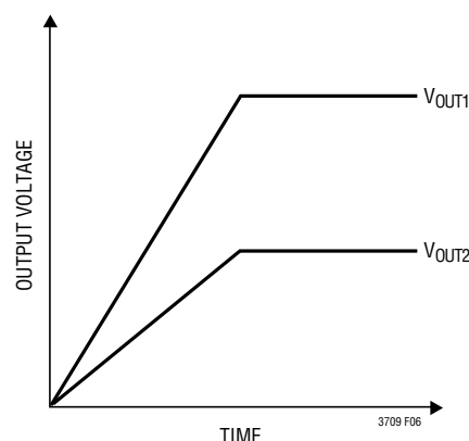
(6b) Ratiometric Tracking
