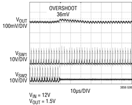
Stage Shedding Transition, 2-Phase to 1-Phase
